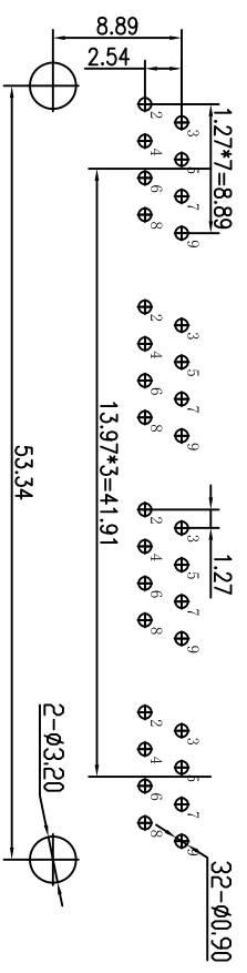
PC Board Layout
