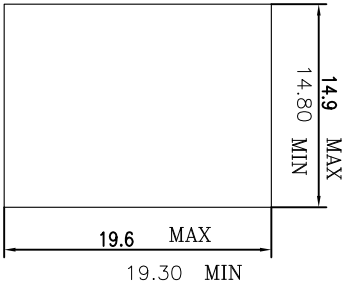
Panel Thickness 1.60mm Single Panel-Latch Clearance
