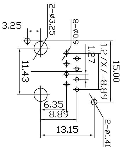
PC Board Layout Component Side Shows
